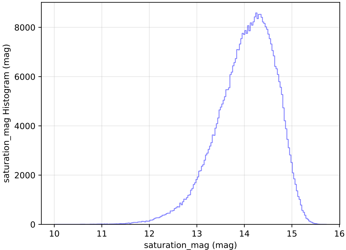
too_ignore_5_4v3.4_10yrs All sky z band: saturation_mag Histogram
