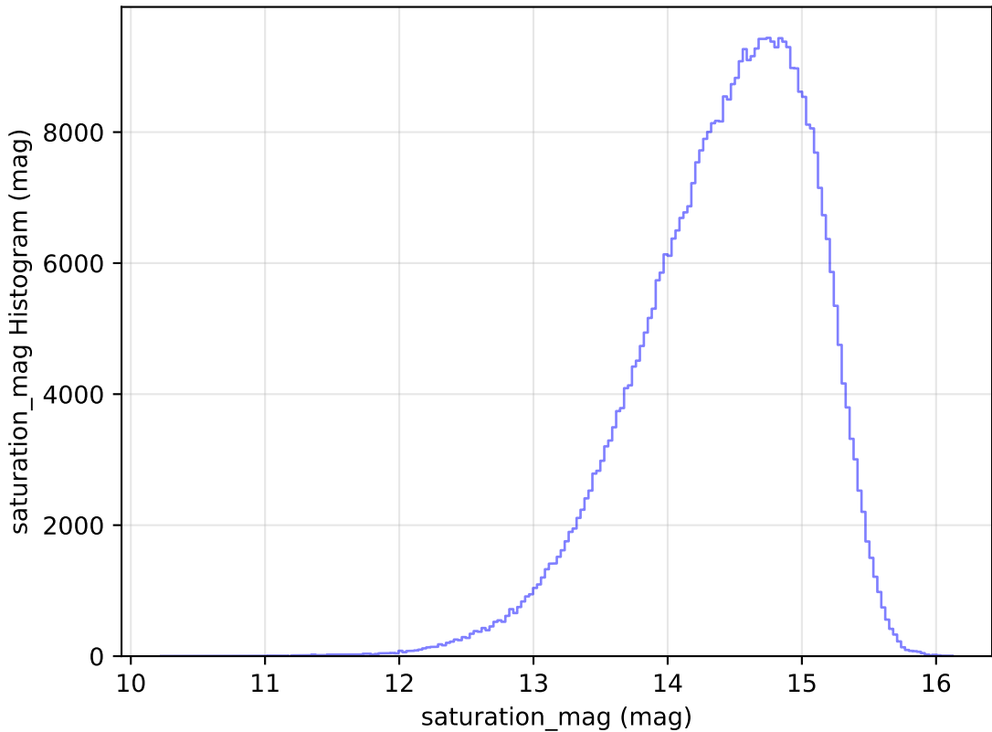
too_ignore_5_4v3.4_10yrs All sky i band: saturation_mag Histogram
