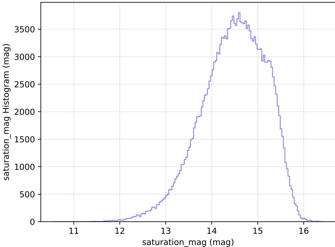
too_ignore_5_4v3.4_10yrs All sky g band: saturation_mag Histogram
