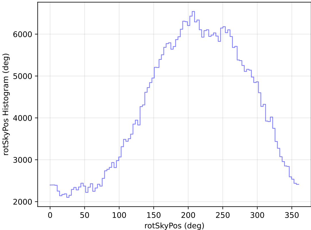
too_ignore_5_4v3.4_10yrs WFD z band: rotSkyPos Histogram
