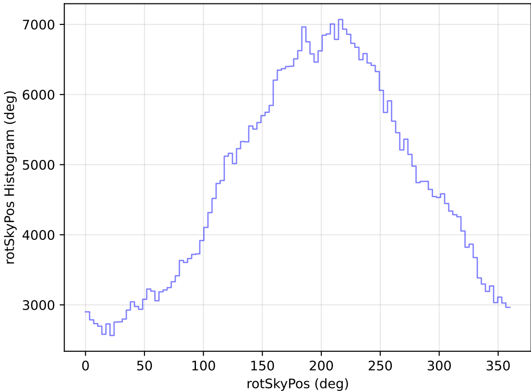
too_ignore_5_4v3.4_10yrs WFD r band: rotSkyPos Histogram
