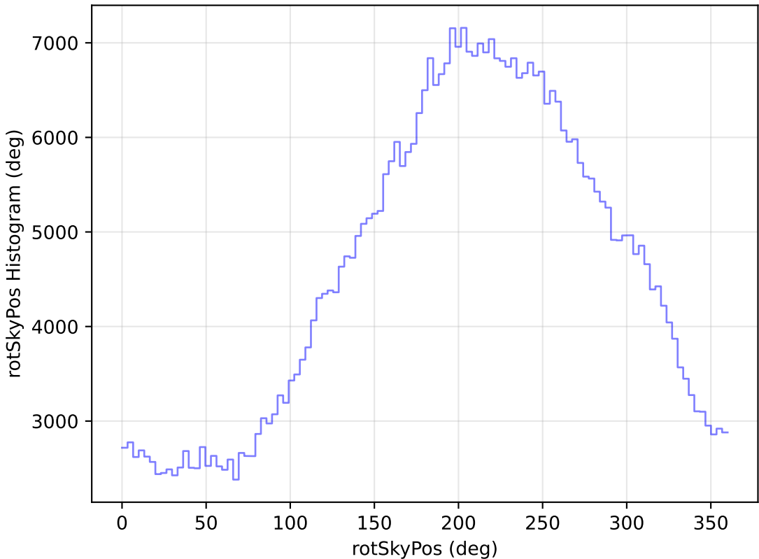
too_ignore_5_4v3.4_10yrs WFD i band: rotSkyPos Histogram
