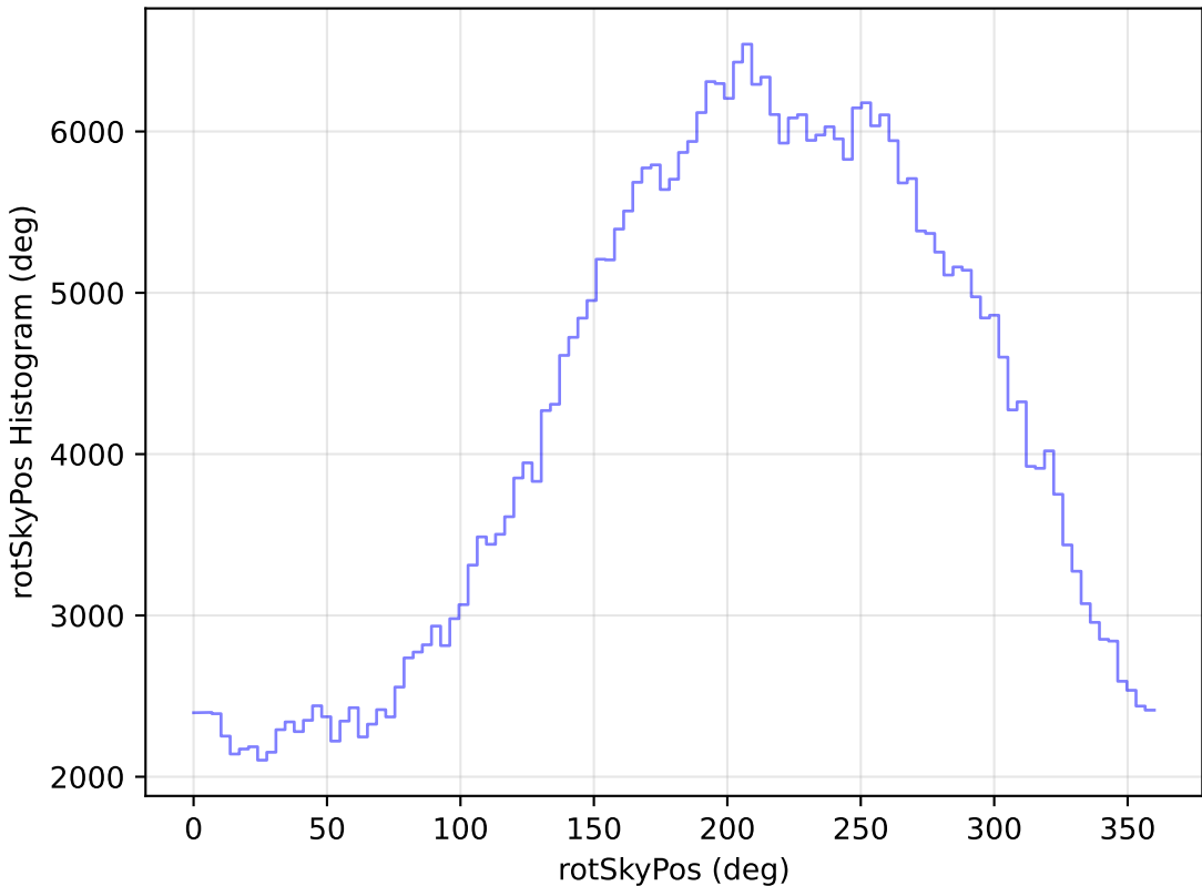
too_ignore_5_4v3.4_10yrs All sky z band: rotSkyPos Histogram
