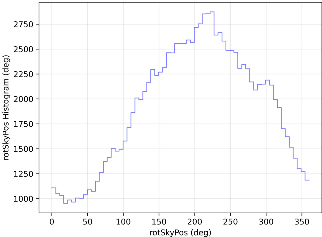
too_ignore_5_4v3.4_10yrs All sky u band: rotSkyPos Histogram
