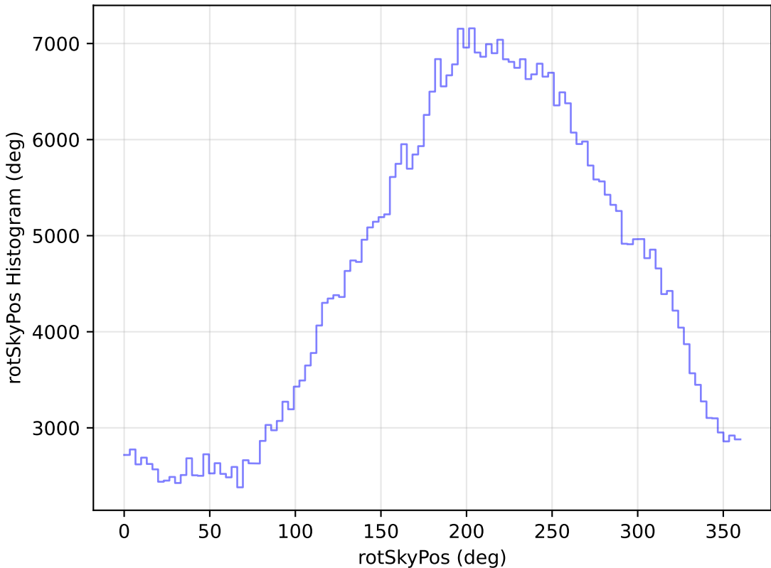
too_ignore_5_4v3.4_10yrs All sky i band: rotSkyPos Histogram
