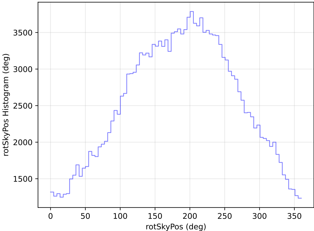
too_ignore_5_4v3.4_10yrs All sky g band: rotSkyPos Histogram
