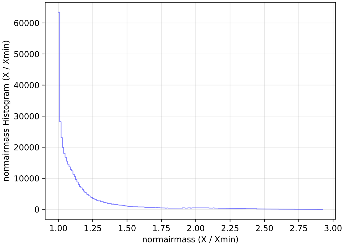
too_ignore_5_4v3.4_10yrs WFD z band: normairmass Histogram
