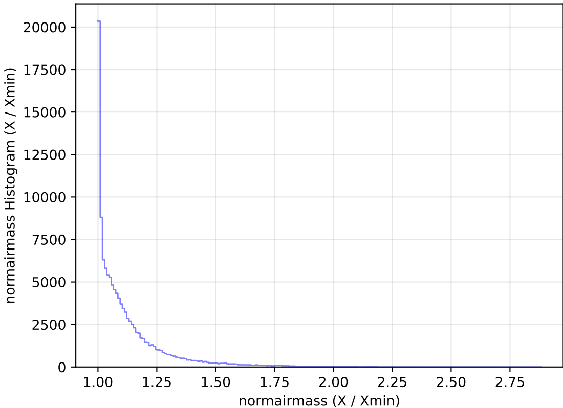
too_ignore_5_4v3.4_10yrs WFD u band: normairmass Histogram
