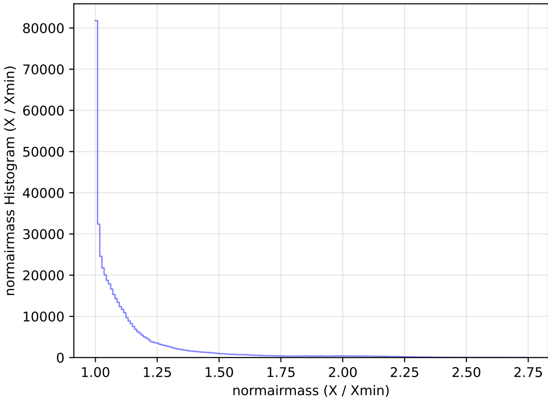
too_ignore_5_4v3.4_10yrs WFD r band: normairmass Histogram
