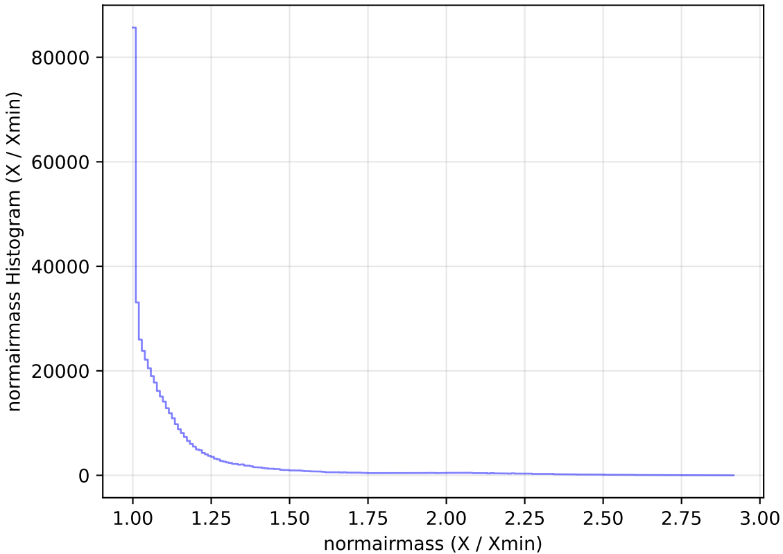
too_ignore_5_4v3.4_10yrs WFD i band: normairmass Histogram
