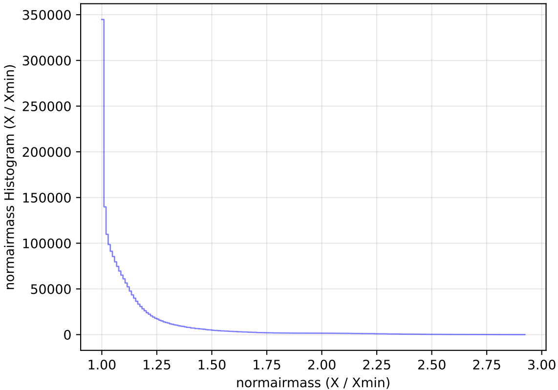
too_ignore_5_4v3.4_10yrs WFD all bands: normairmass Histogram
