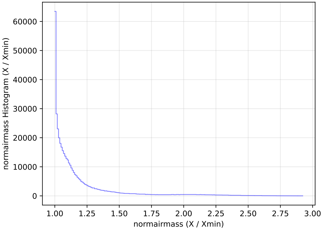
too_ignore_5_4v3.4_10yrs All sky z band: normairmass Histogram
