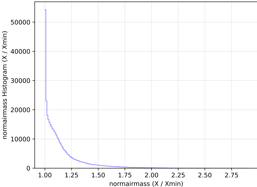
too_ignore_5_4v3.4_10yrs All sky y band: normairmass Histogram
