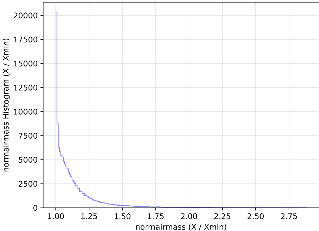
too_ignore_5_4v3.4_10yrs All sky u band: normairmass Histogram
