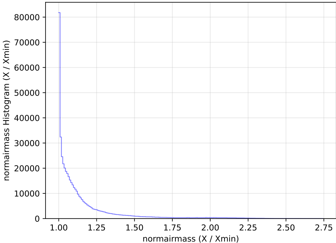
too_ignore_5_4v3.4_10yrs All sky r band: normairmass Histogram
