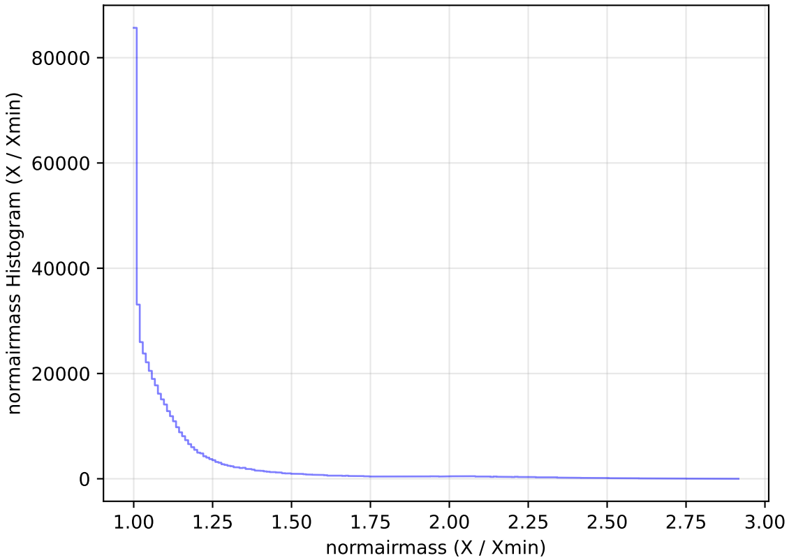
too_ignore_5_4v3.4_10yrs All sky i band: normairmass Histogram
