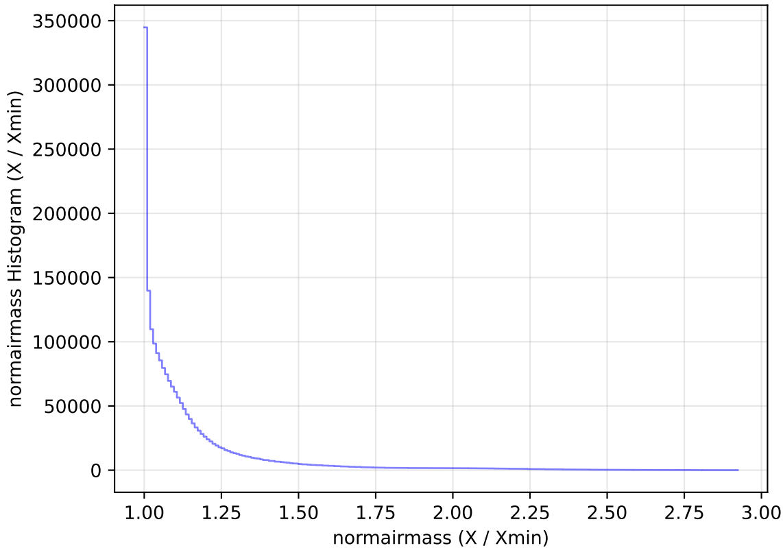
too_ignore_5_4v3.4_10yrs All sky all bands: normairmass Histogram
