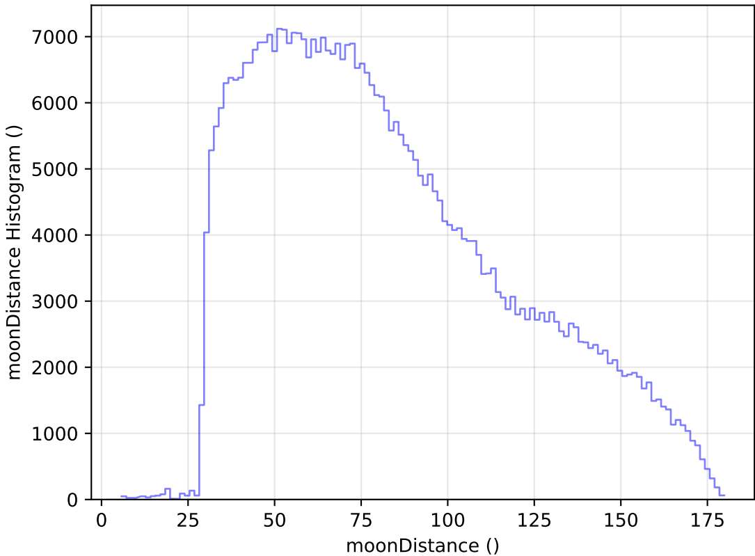
too_ignore_5_4v3.4_10yrs WFD z band: moonDistance Histogram
