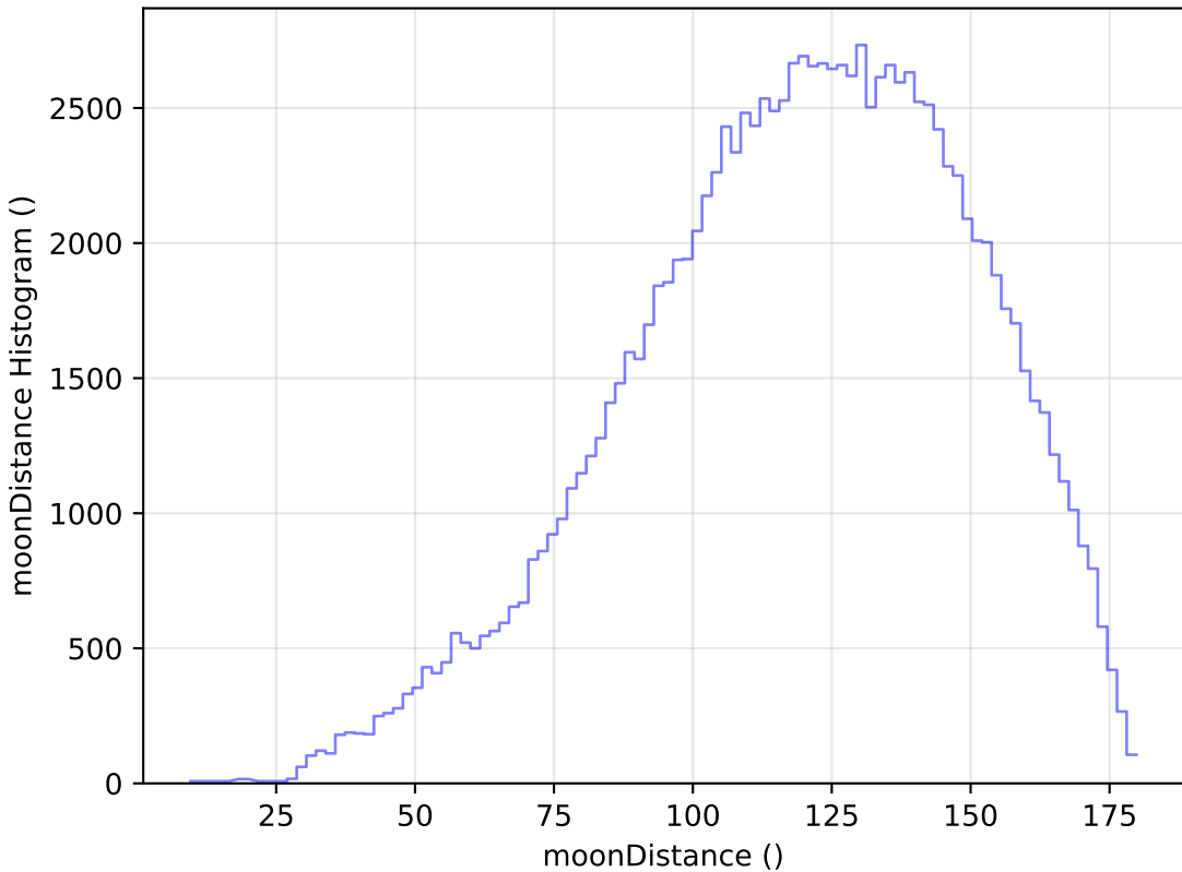
too_ignore_5_4v3.4_10yrs WFD u band: moonDistance Histogram
