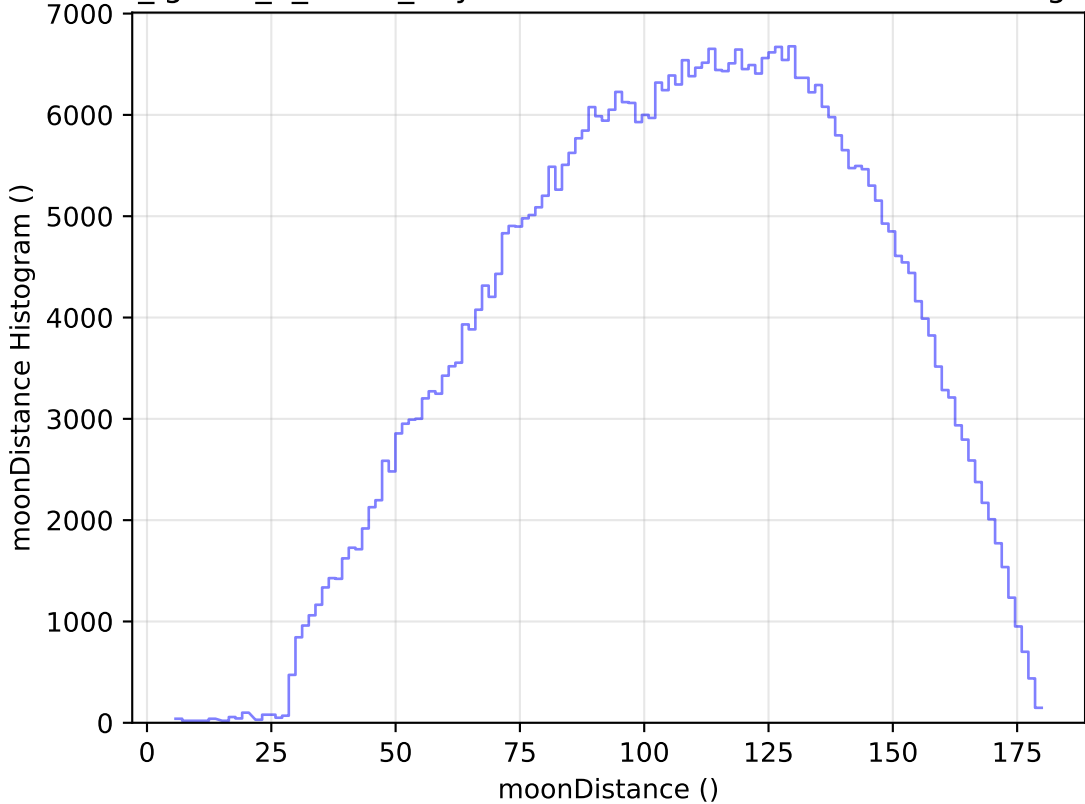
too_ignore_5_4v3.4_10yrs WFD r band: moonDistance Histogram
