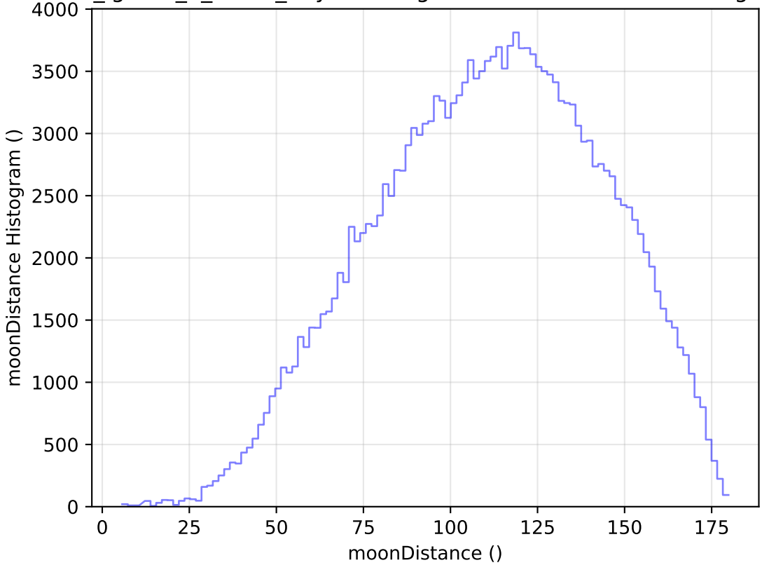
too_ignore_5_4v3.4_10yrs WFD g band: moonDistance Histogram
