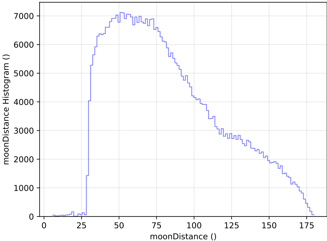
too_ignore_5_4v3.4_10yrs All sky z band: moonDistance Histogram
