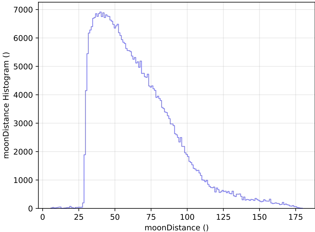
too_ignore_5_4v3.4_10yrs All sky y band: moonDistance Histogram
