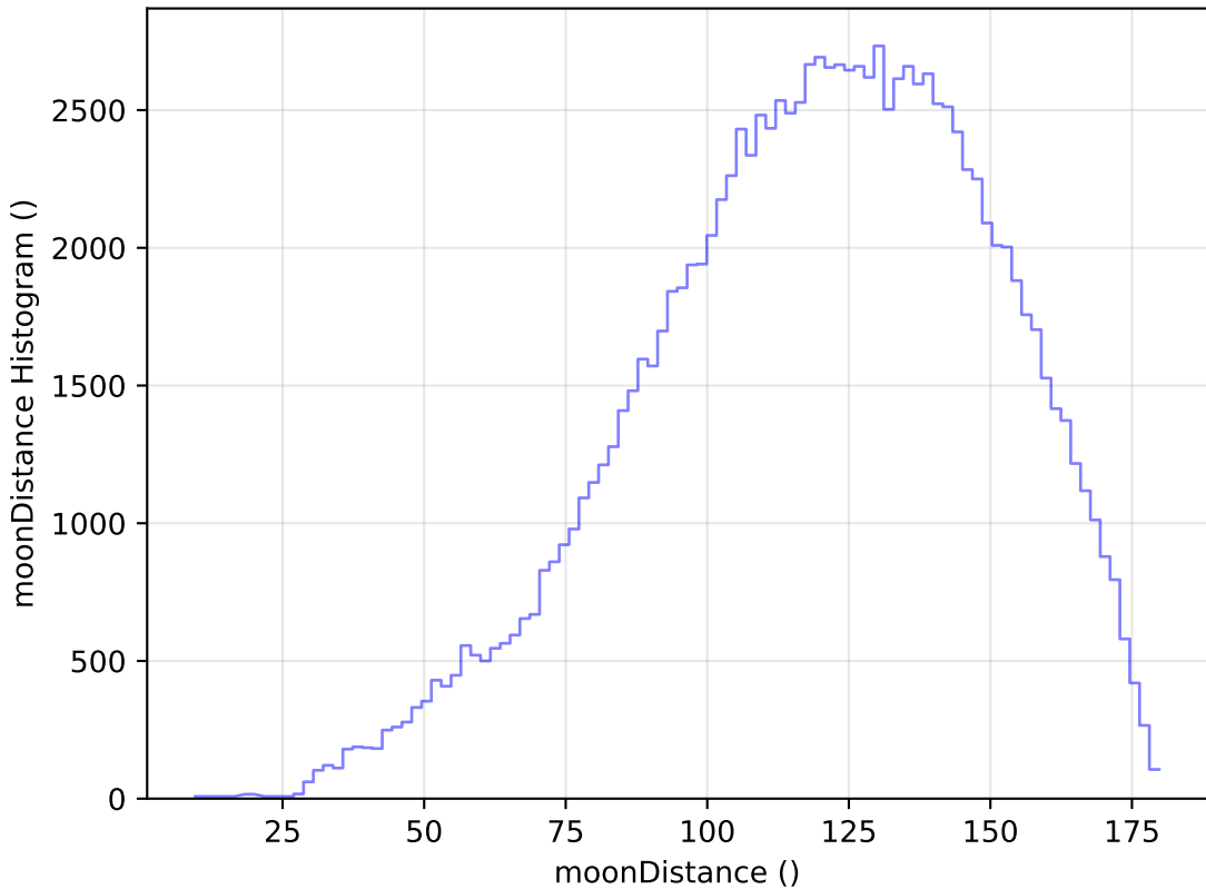
too_ignore_5_4v3.4_10yrs All sky u band: moonDistance Histogram
