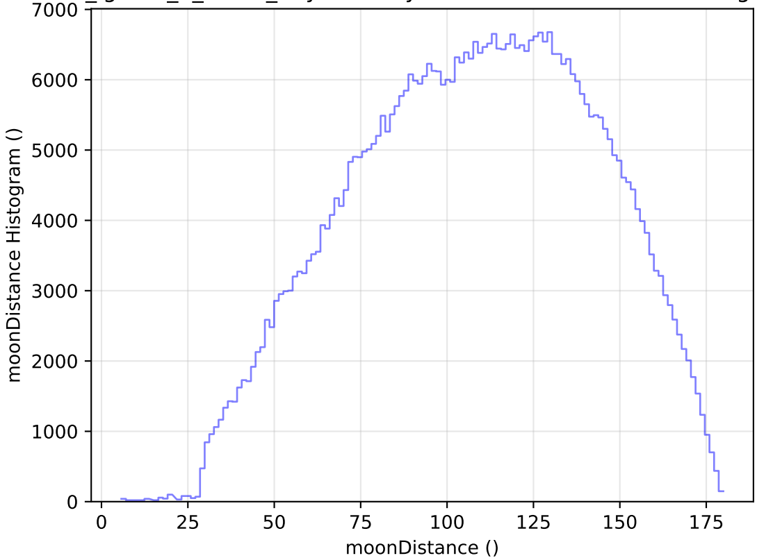
too_ignore_5_4v3.4_10yrs All sky r band: moonDistance Histogram
