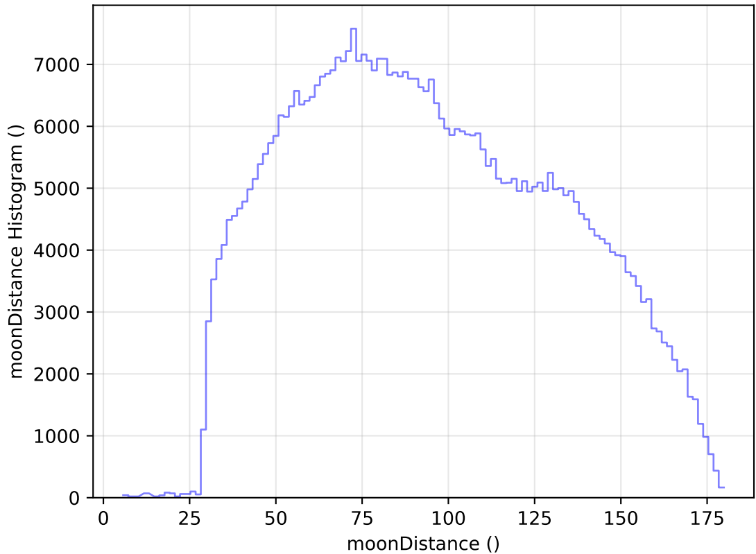
too_ignore_5_4v3.4_10yrs All sky i band: moonDistance Histogram
