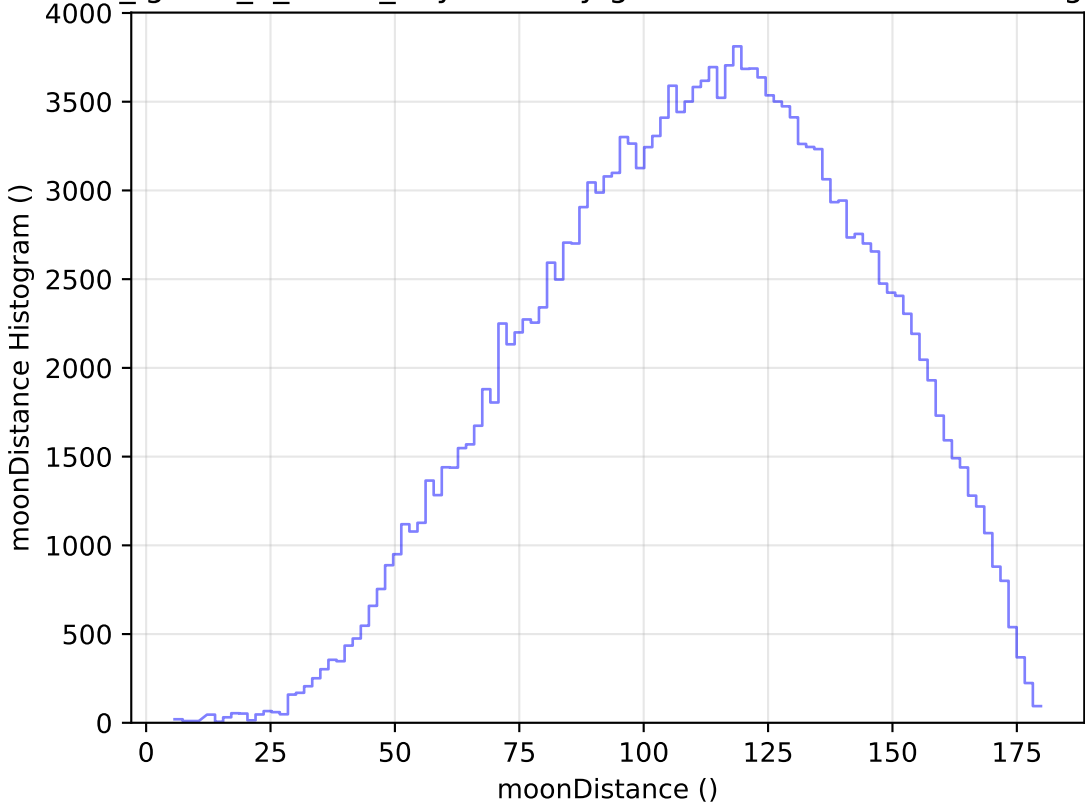
too_ignore_5_4v3.4_10yrs All sky g band: moonDistance Histogram
