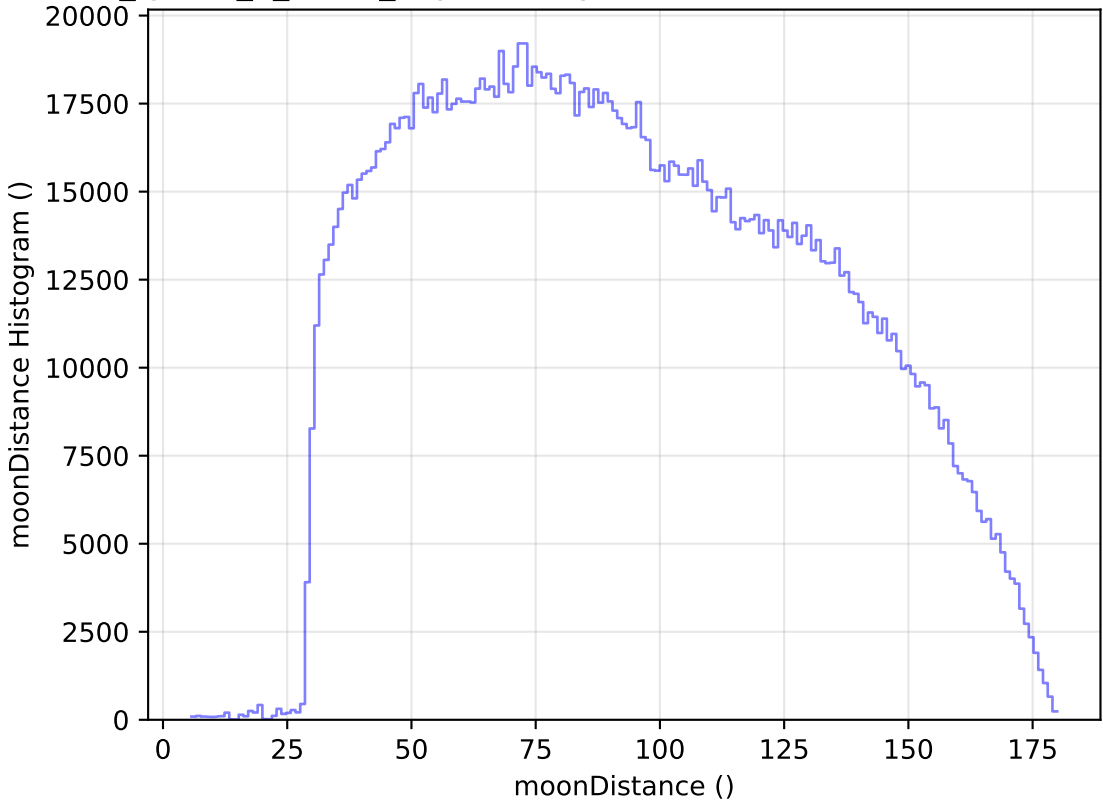
too_ignore_5_4v3.4_10yrs All sky all bands: moonDistance Histogram
