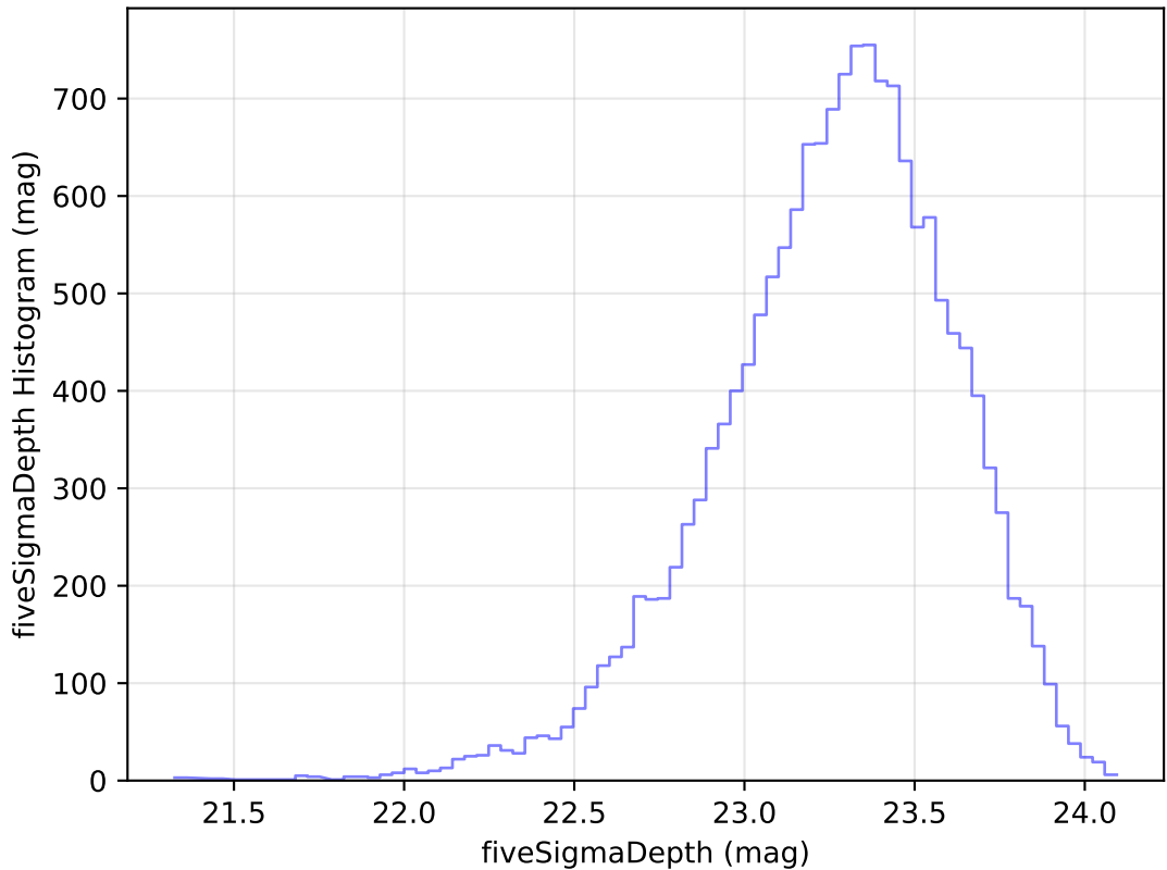
too_ignore_5_4v3.4_10yrs Yr 1 u band: fiveSigmaDepth Histogram
