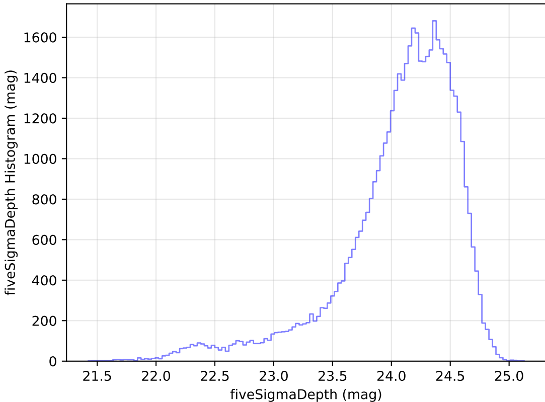
too_ignore_5_4v3.4_10yrs Yr 1 r band: fiveSigmaDepth Histogram
