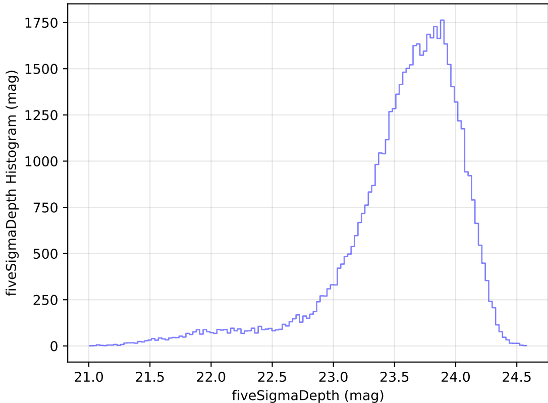
too_ignore_5_4v3.4_10yrs Yr 1 i band: fiveSigmaDepth Histogram
