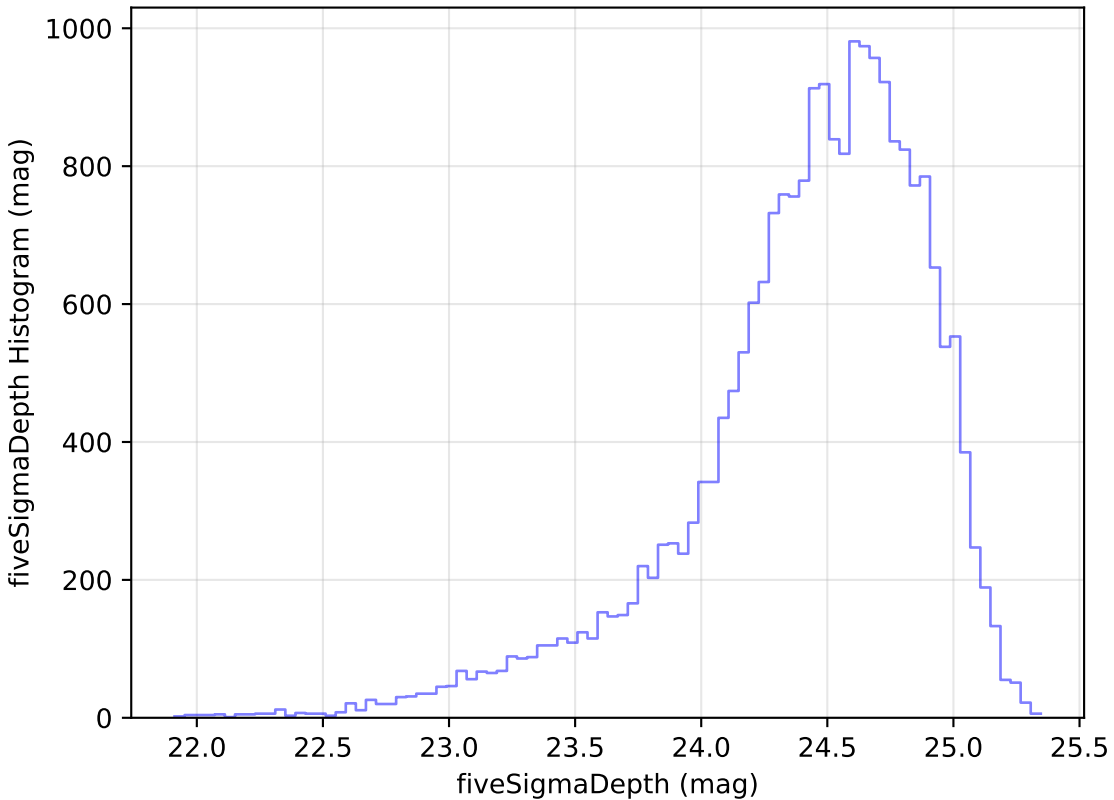
too_ignore_5_4v3.4_10yrs Yr 1 g band: fiveSigmaDepth Histogram
