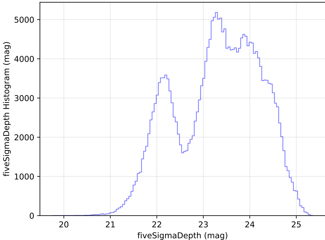
too_ignore_5_4v3.4_10yrs Yr 1 all bands: fiveSigmaDepth Histogram
