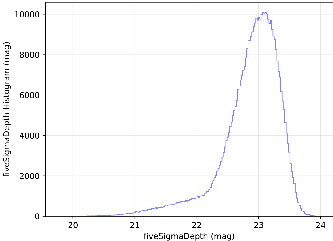
too_ignore_5_4v3.4_10yrs WFD z band: fiveSigmaDepth Histogram
