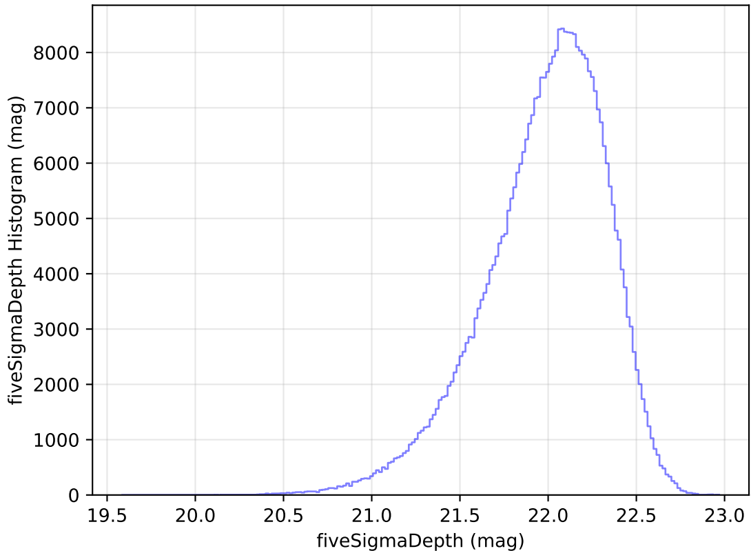
too_ignore_5_4v3.4_10yrs WFD y band: fiveSigmaDepth Histogram
