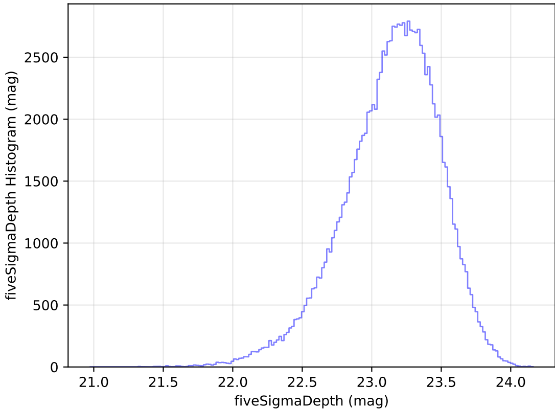
too_ignore_5_4v3.4_10yrs WFD u band: fiveSigmaDepth Histogram
