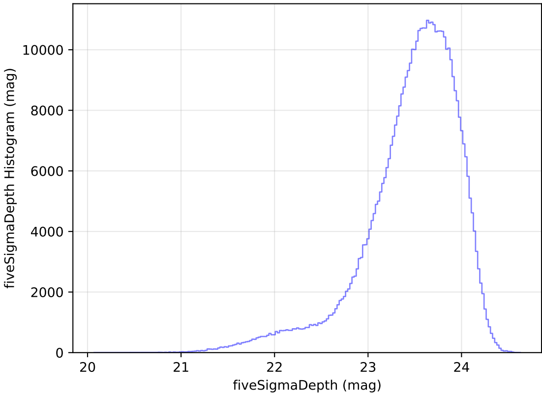
too_ignore_5_4v3.4_10yrs WFD i band: fiveSigmaDepth Histogram
