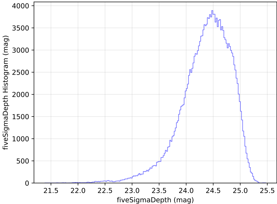
too_ignore_5_4v3.4_10yrs WFD g band: fiveSigmaDepth Histogram
