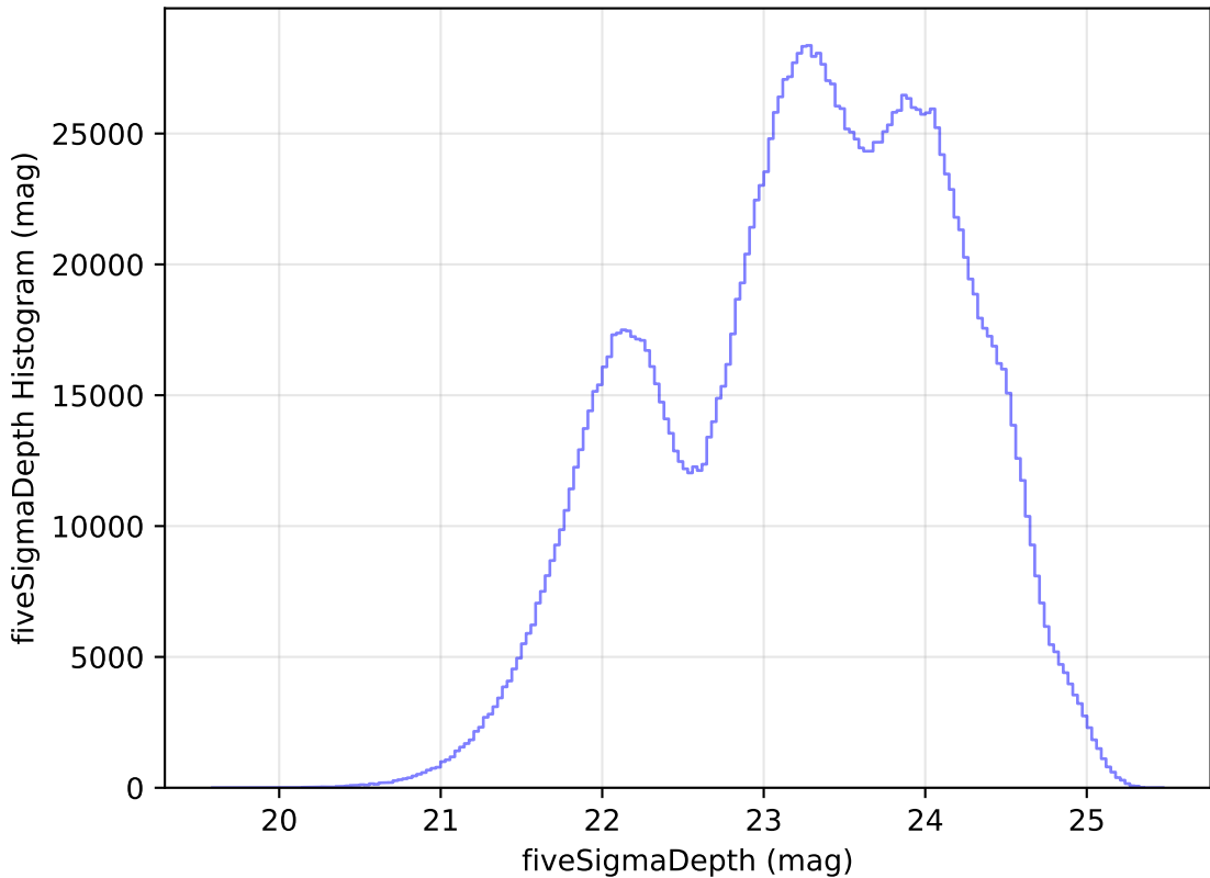
too_ignore_5_4v3.4_10yrs WFD all bands: fiveSigmaDepth Histogram
