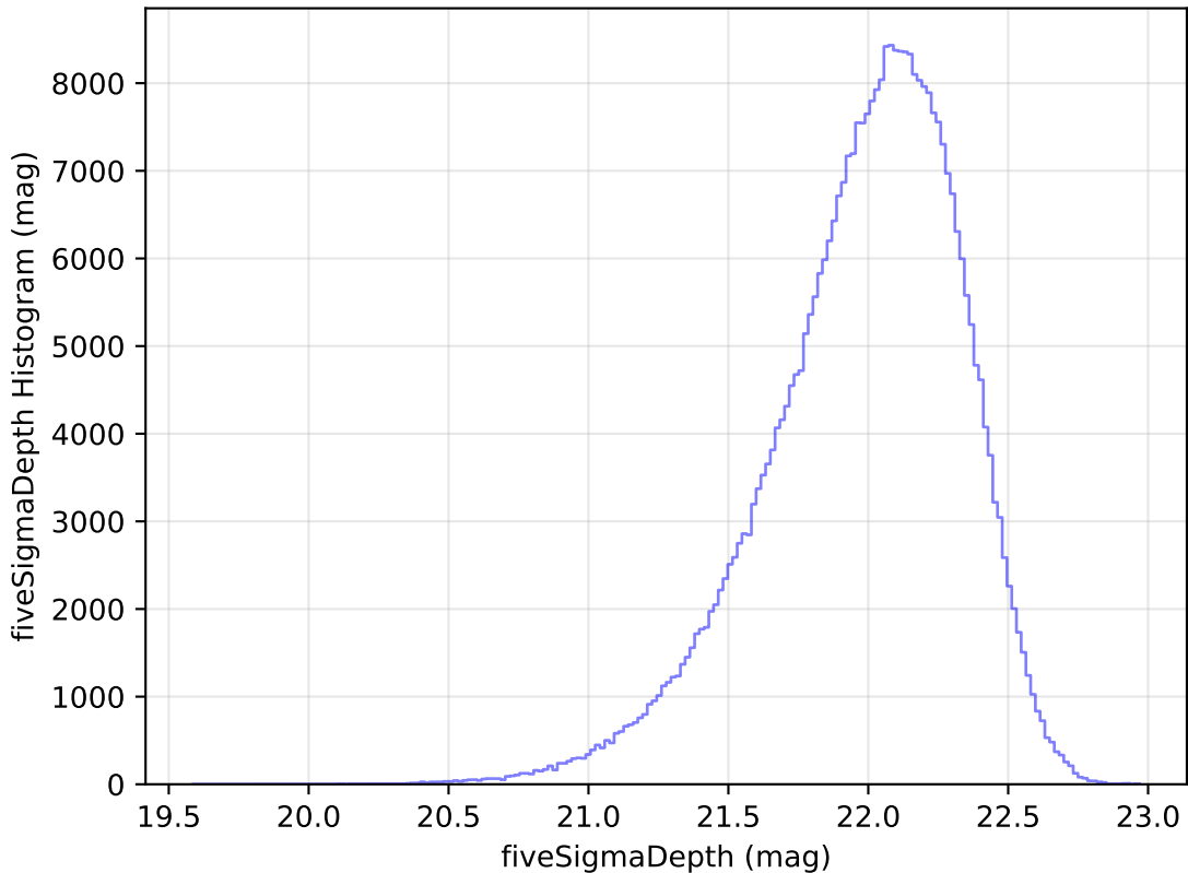
too_ignore_5_4v3.4_10yrs All sky y band: fiveSigmaDepth Histogram
