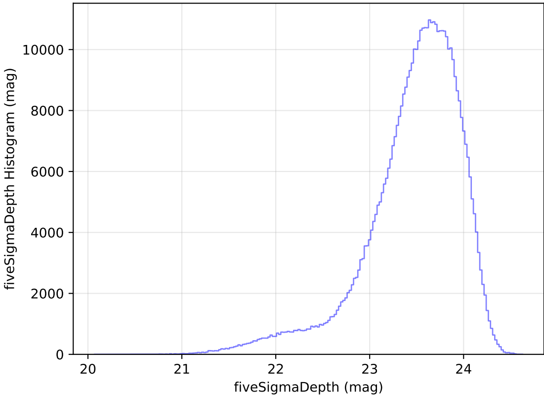
too_ignore_5_4v3.4_10yrs All sky i band: fiveSigmaDepth Histogram
