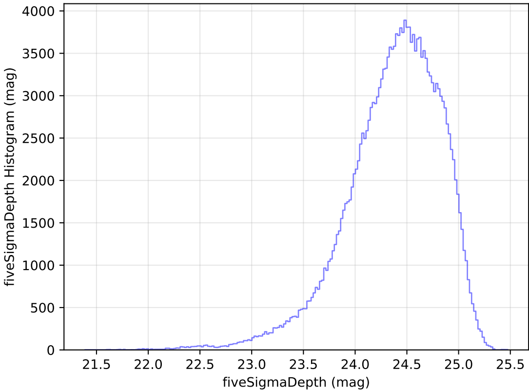
too_ignore_5_4v3.4_10yrs All sky g band: fiveSigmaDepth Histogram
