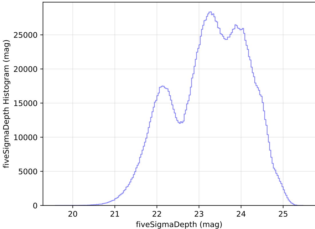
too_ignore_5_4v3.4_10yrs All sky all bands: fiveSigmaDepth Histogram
