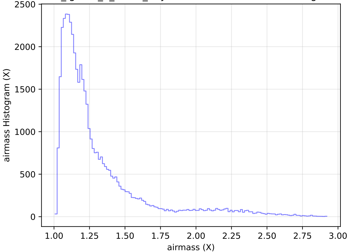
too_ignore_5_4v3.4_10yrs Yr 1 z band: airmass Histogram
