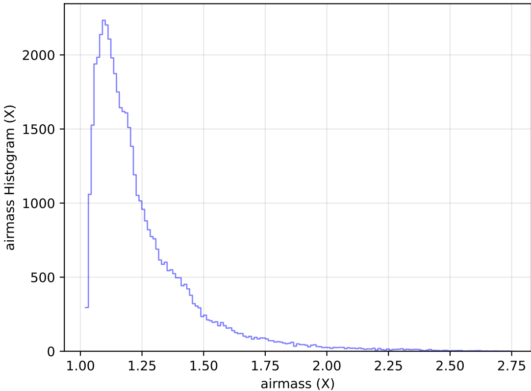
too_ignore_5_4v3.4_10yrs Yr 1 y band: airmass Histogram
