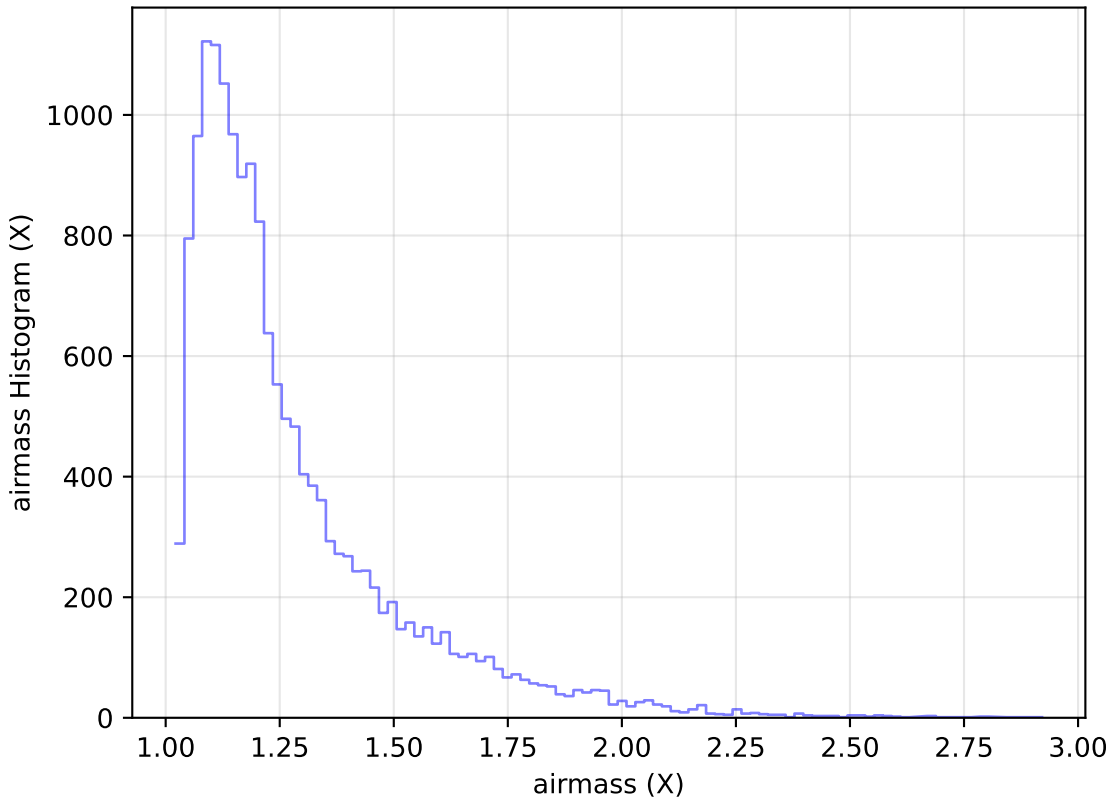
too_ignore_5_4v3.4_10yrs Yr 1 u band: airmass Histogram
